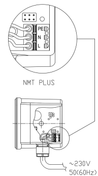
Electrical drawing
