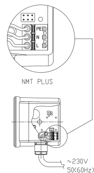
Electrical drawing
