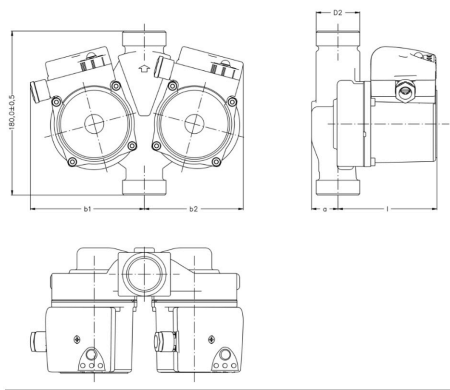
Dimension drawing
